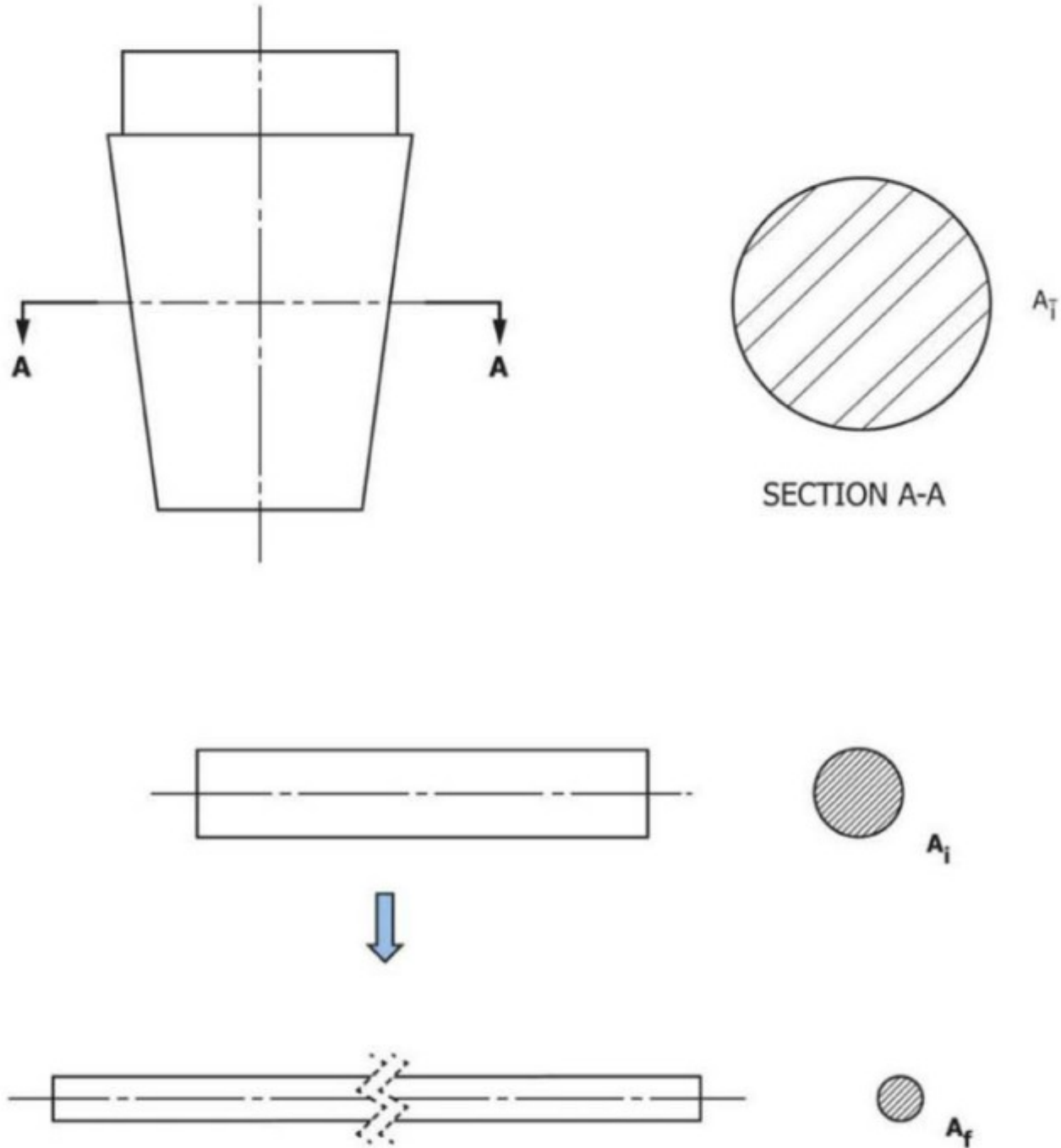
FIG. X1.1 Solid Forging
