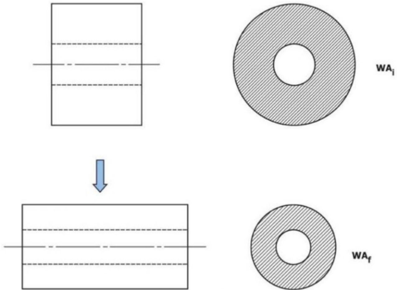
FIG. X1.2 Hollow Forging
